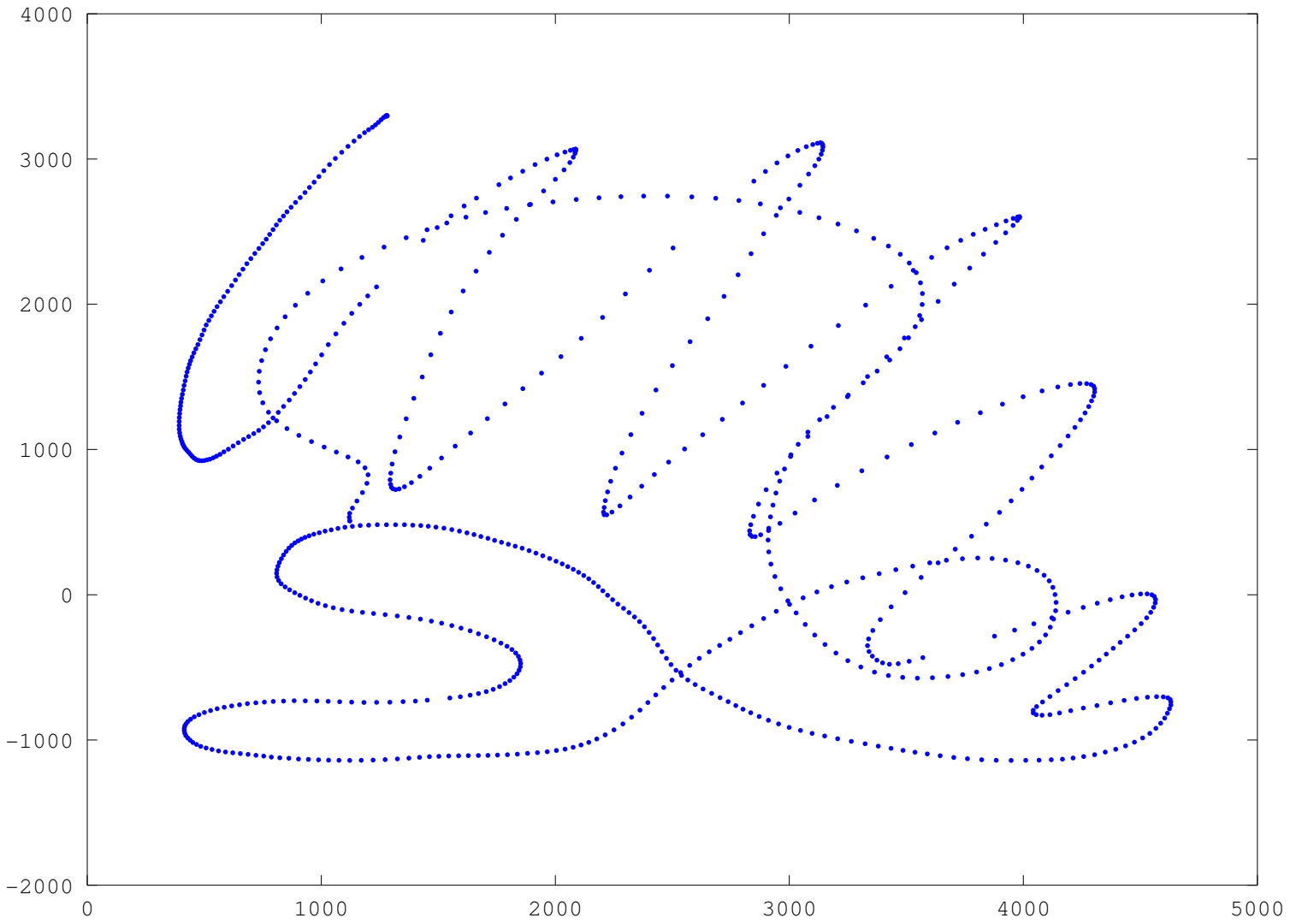
Painting trajectory
